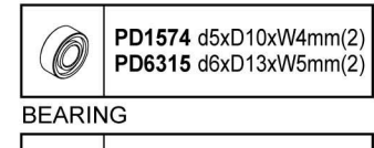
BEARING
