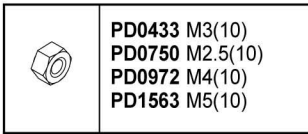
LOCK NUT
